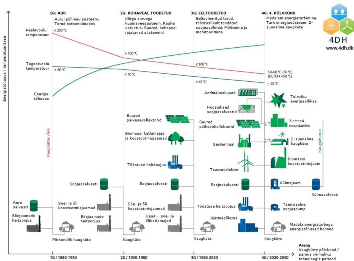
Joonis 2.1. Kaugkütte põlvkonnad (allikas: Thorsen, J. E., Lund, H., & Mathiesen, B. V. (2018). "Progression of District Heating – 1st to 4th generation")
